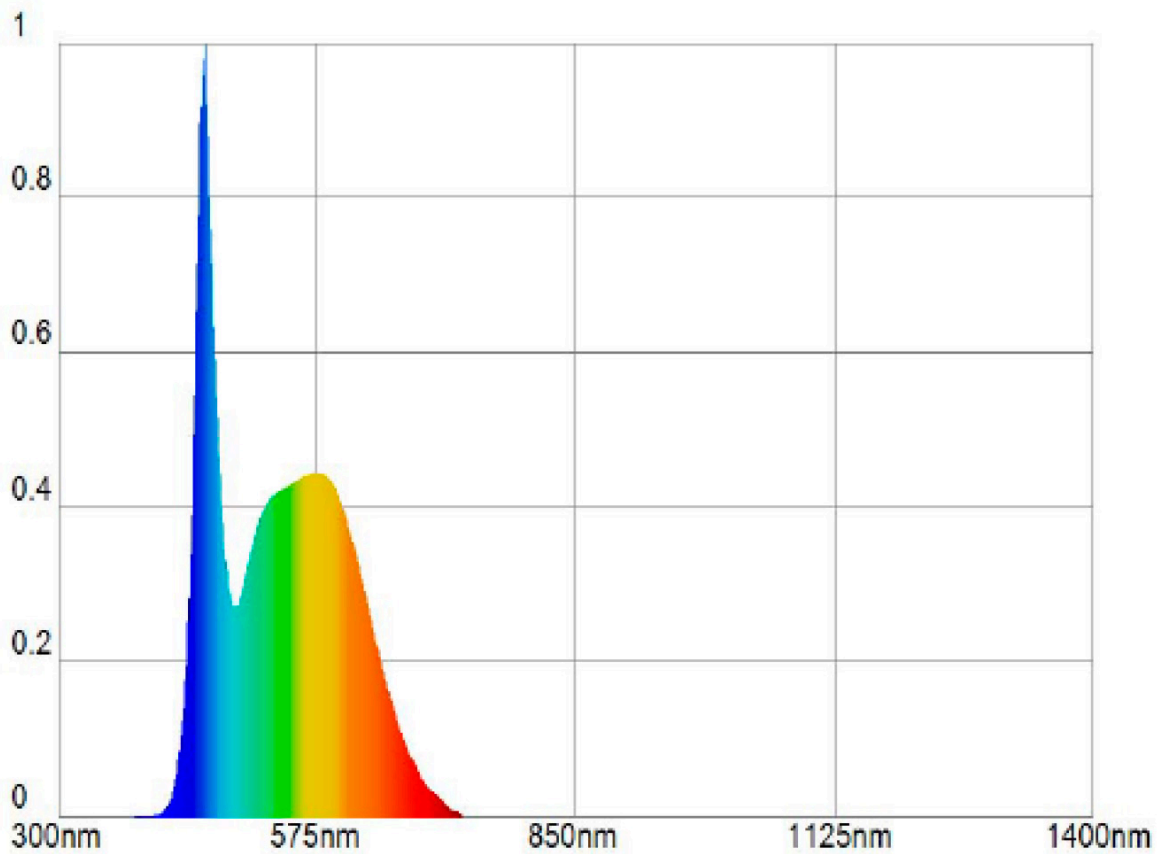
Measured spectral radiance distribution
