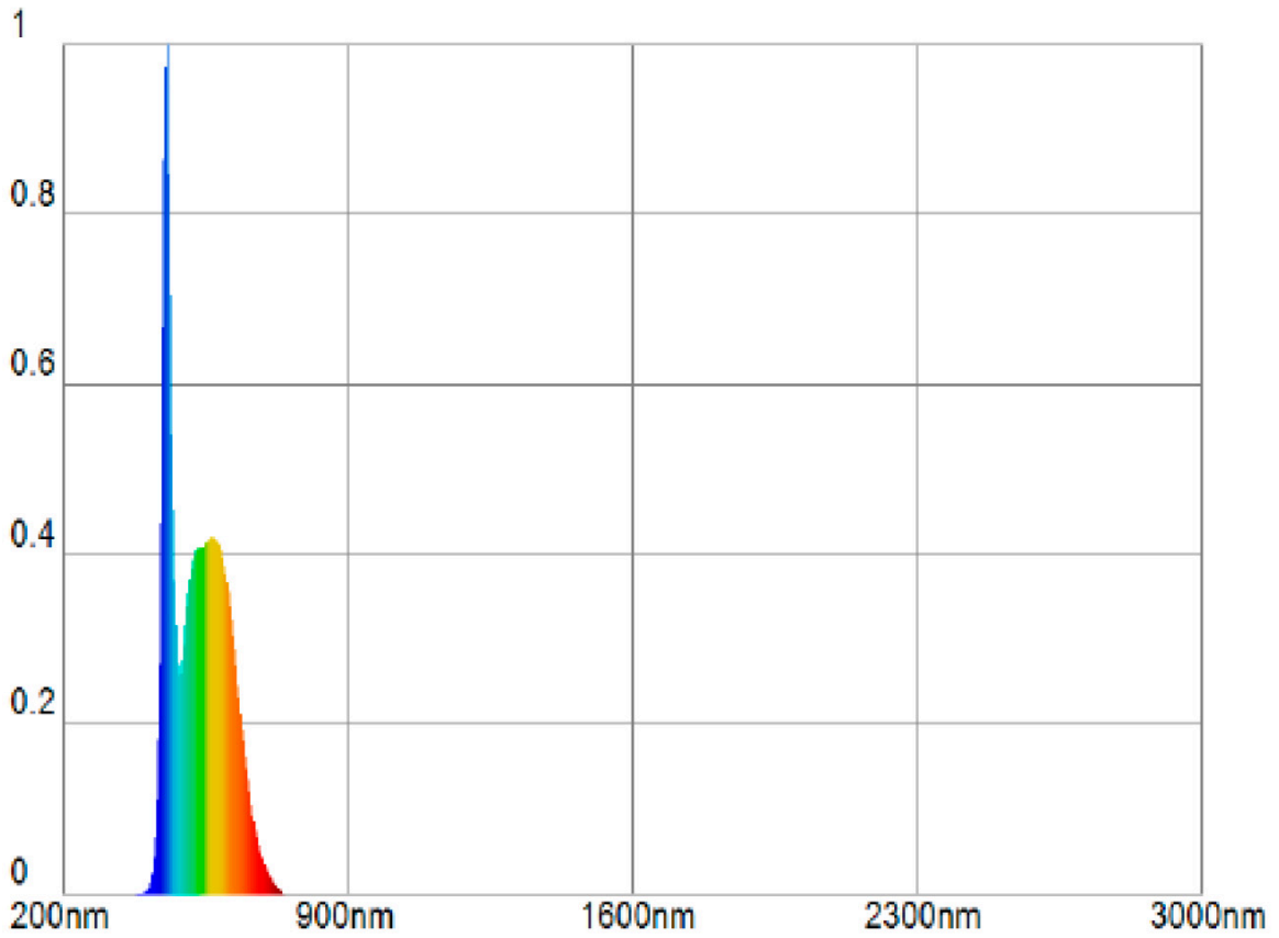
Measured spectral irradiance distribution
